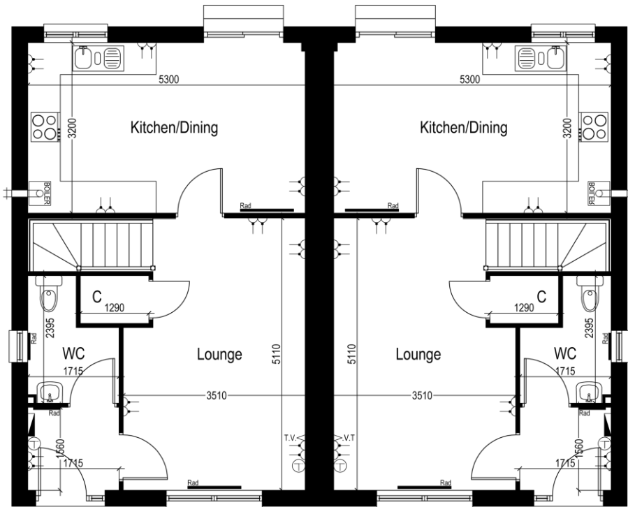
Ground Floor Plan 44.5sqm
